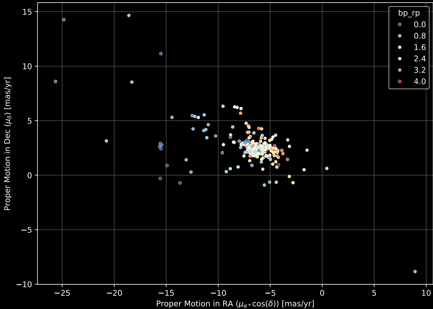
APOGEE DR17 Field: [288-01-C] Proper Motion Diagram (n= 263)
