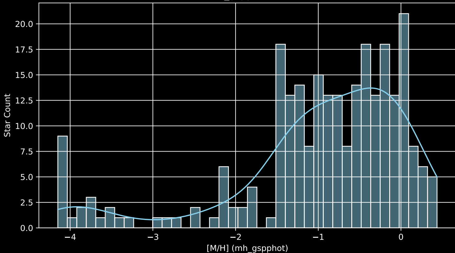
APOGEE DR17 Field: [288-01-C [M/H] (mh_gspphot) (n= 259)
