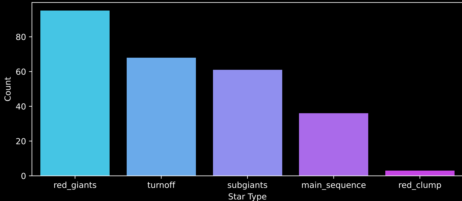
APOGEE DR17 Field: [288-01-C] Count plot of Star Type
