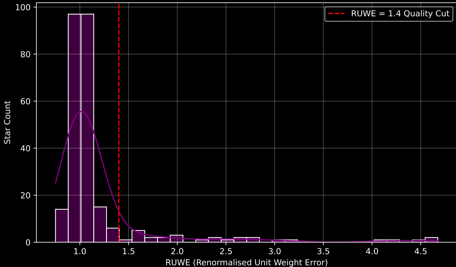
GAPOGEE DR17 Field [288-01-C] RUWE Distribution (n= 257)
