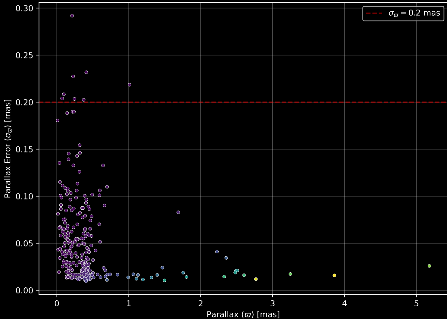
APOGEE DR17 Field: [288-01-C] Parallax Quality (n= 263)
