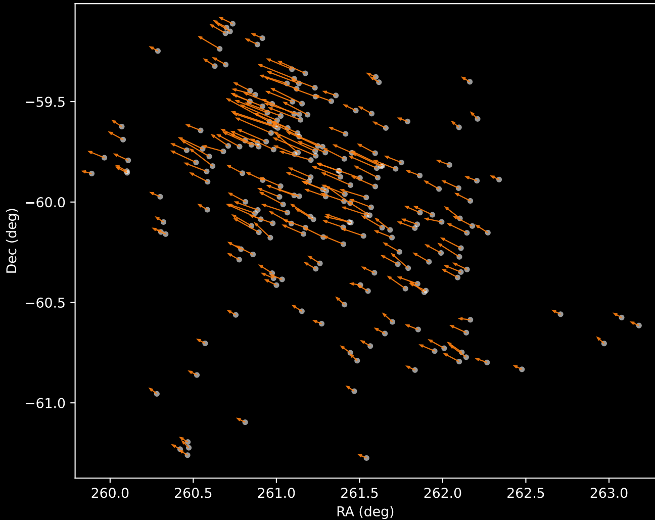
APOGEE DR17 Cluster 2 Proper Motion Vectors (n=221)
